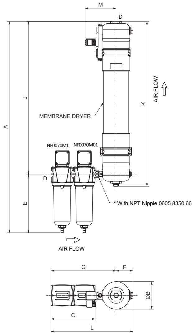
DETAIL: DRYER WITHOUT SOLENOID VALVE
