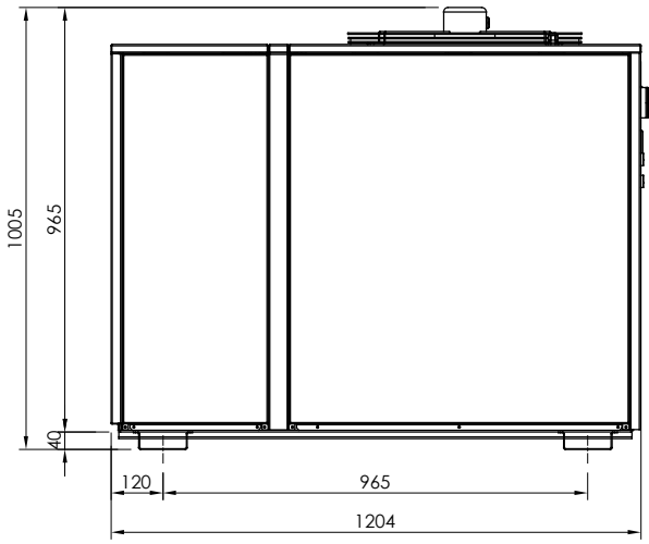
LEFT VIEW
