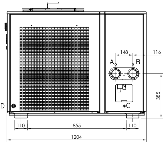
RIGHT VIEW
