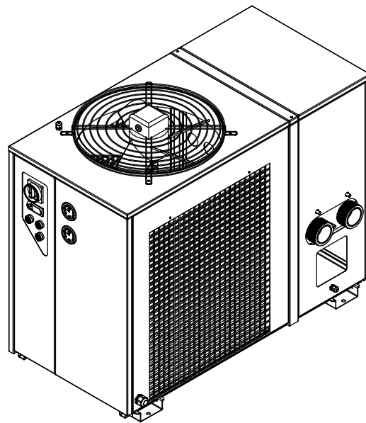
ISOMETRIC VIEW
