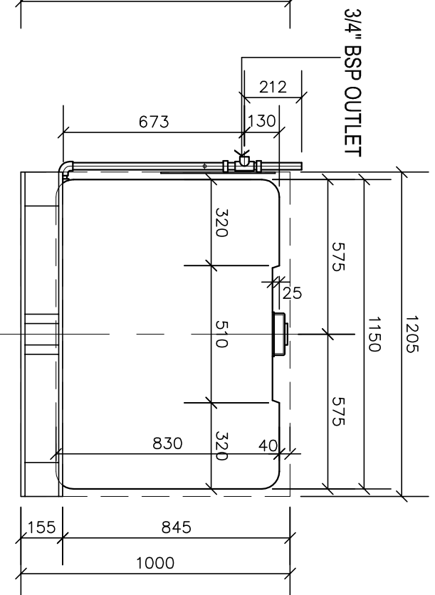
SIDE ELEVATION
