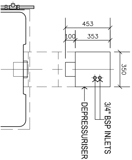
INLET DETAIL
