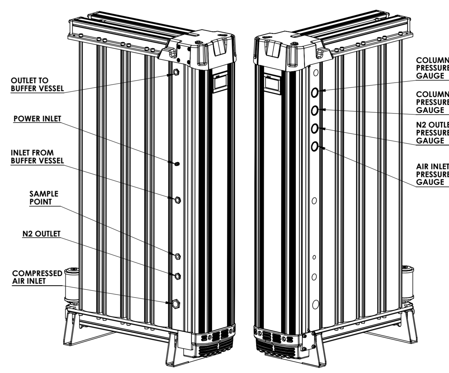
PICTORIAL VIEWS
