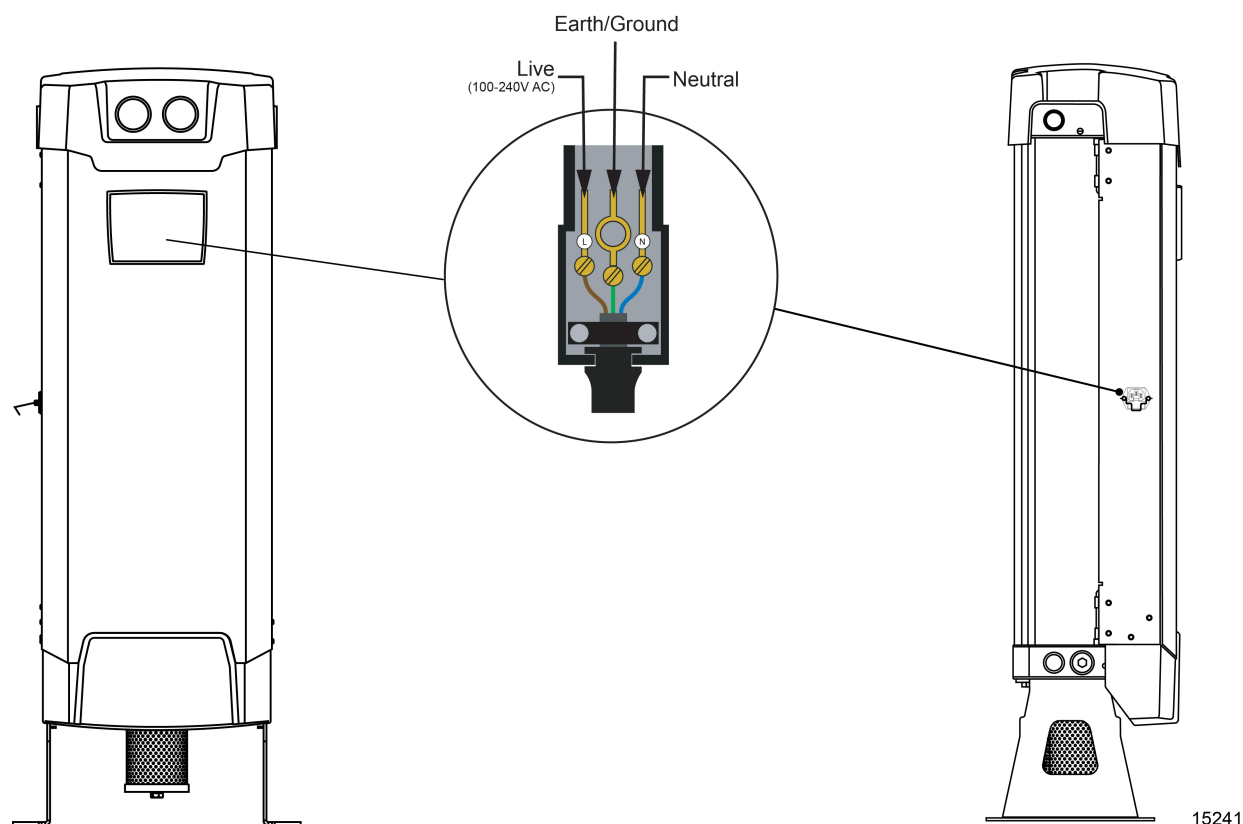
Figure 1: Electrical connections
