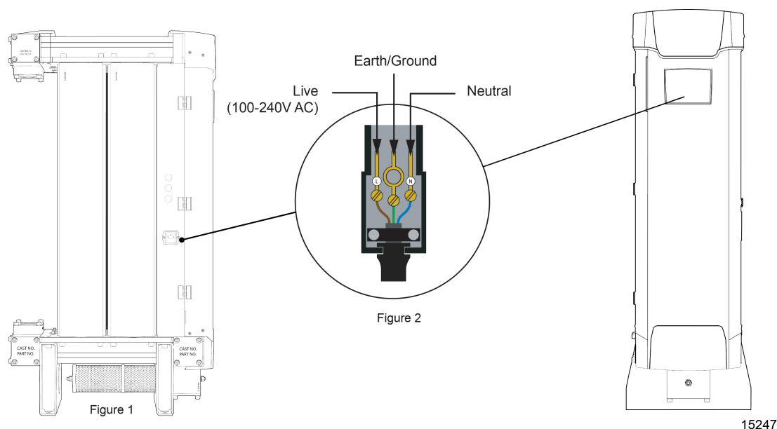
Figure 1: Electrical connections
